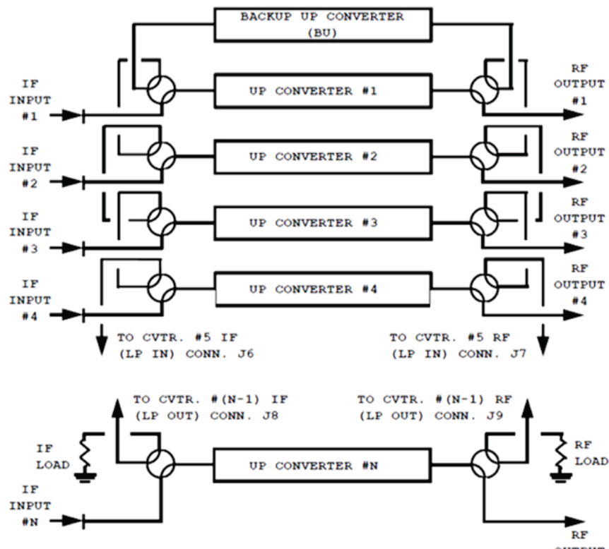
1:N Redundant Configuration Diagram with IOM-XX
