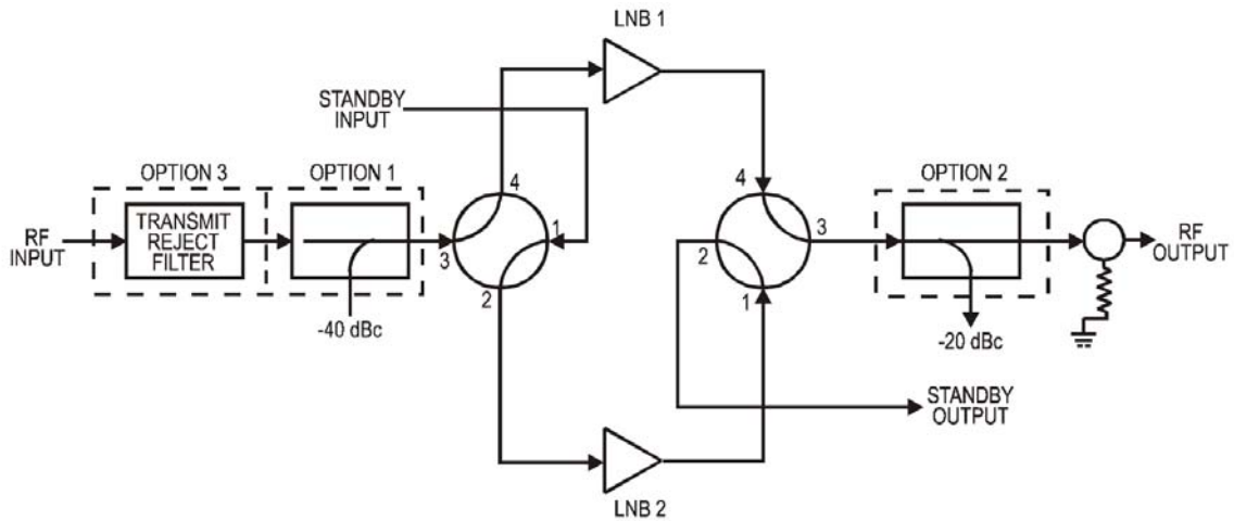
1:2 Redundant LNB System Block Diagram
