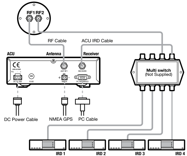
Figure 17 : Multi-IRDs Configuration
