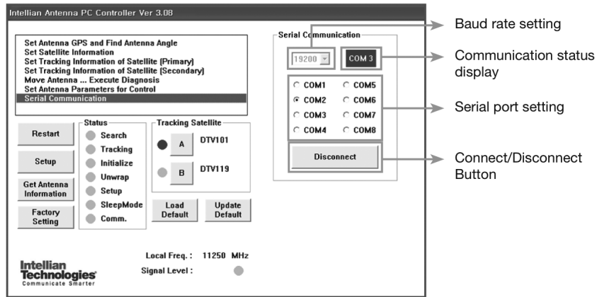
Figure 22 : Setup for Serial Communication
