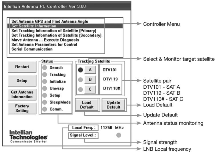
Figure 23 : Setup for Satellite Information in Dual-Sat Mode
