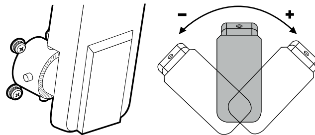
Figure 19 : Manual Angle Adjustment LNB Skew
