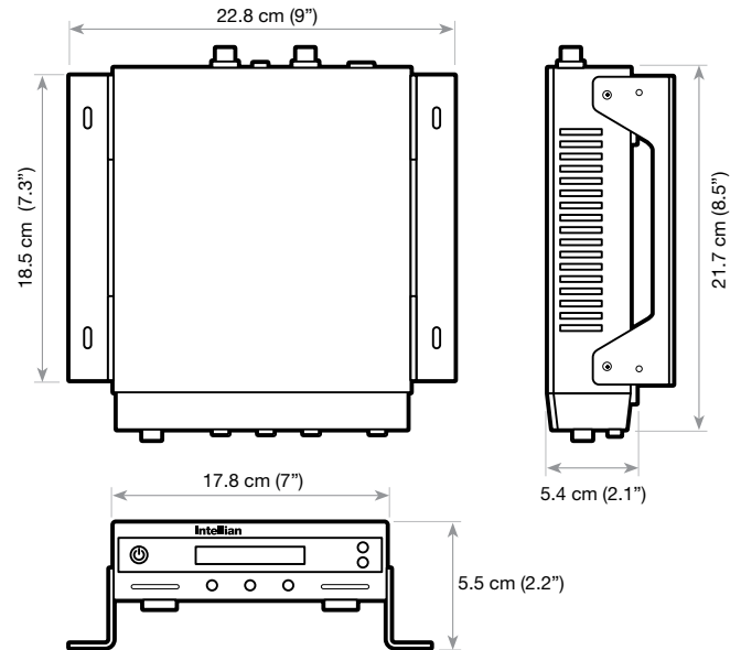
Figure 13 : Dimension of ACU
