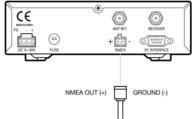
Figure 18 : NMEA 0183 GPS Connection
