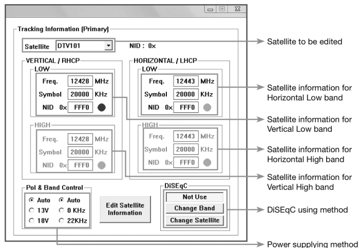
Figure 29 : Setting up the Primary Tracking Information
