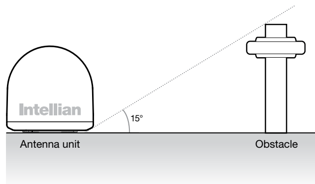
Figure 07 : Elevation Limit of Obstacles
