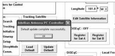
Figure 26 : Updates Completed
