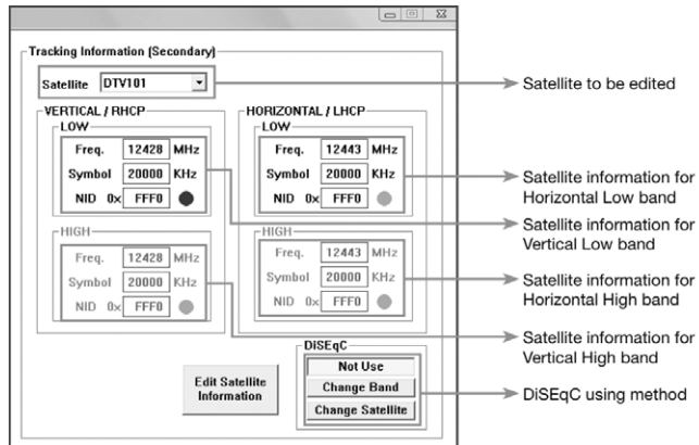
Figure 30 : Setting up the Secondary Tracking Information
