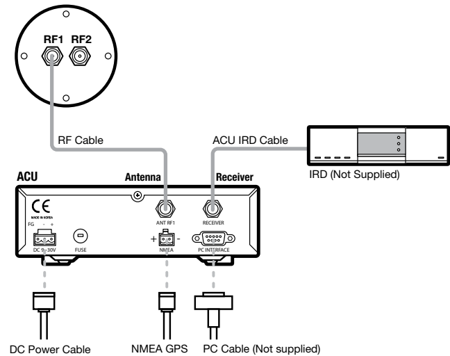
Figure 15 : Single IRD Configuration
