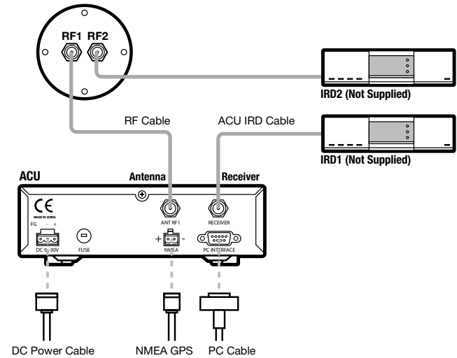
Figure 16 : Dual-IRDs Configuration
