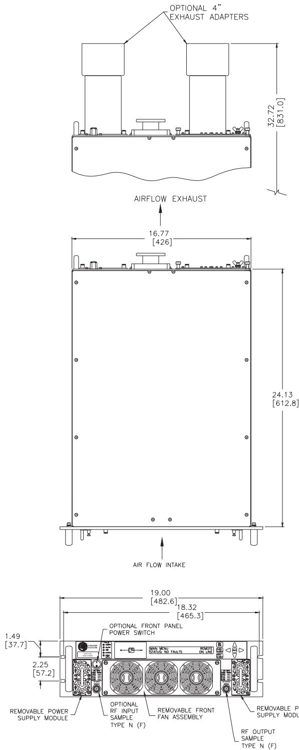
Outline Drawing, 250W C-Band 3RU SSPA Chassis
