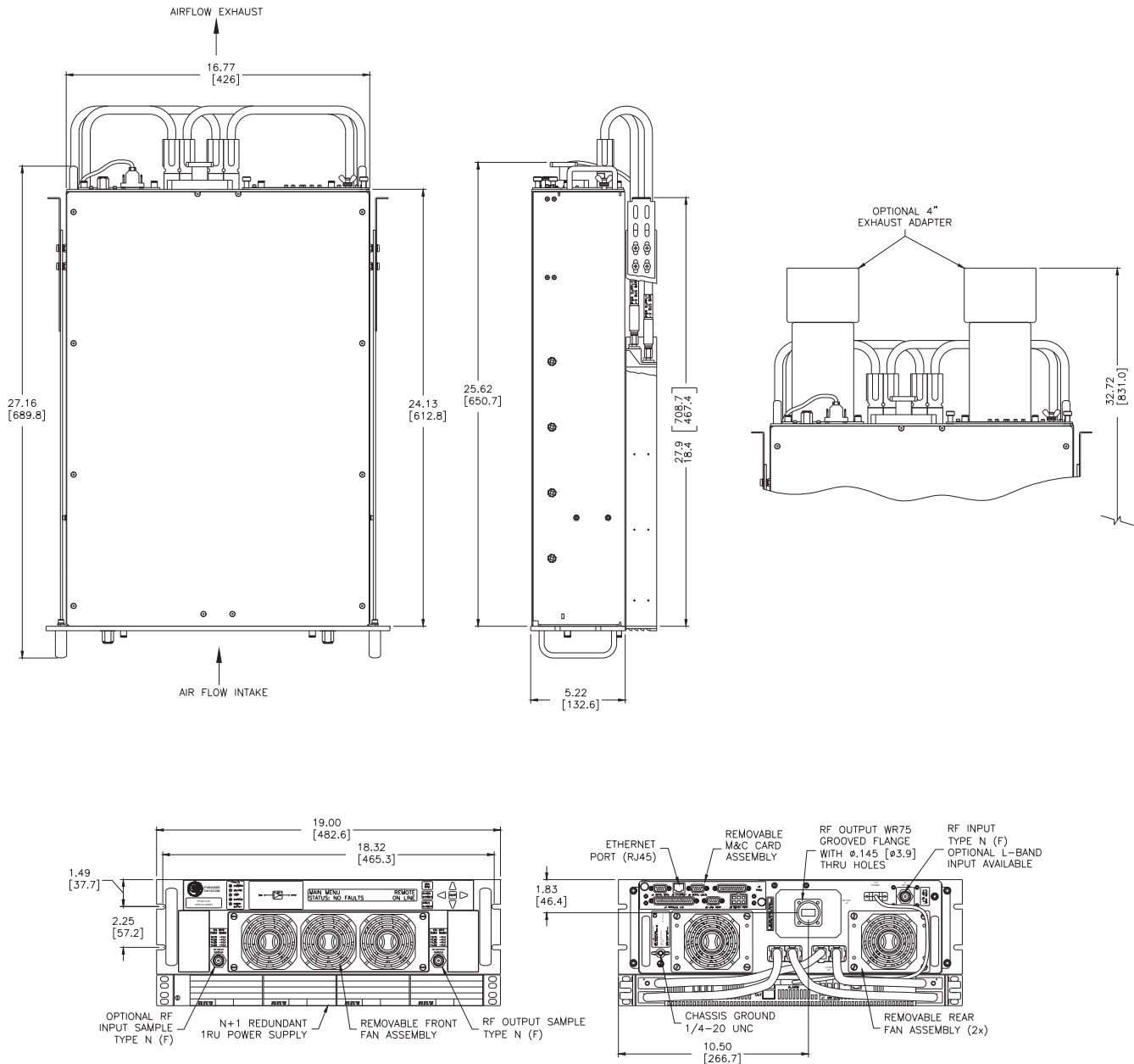
Outline Drawing, 125W Ku-Band 3RU SSPA Chassis with 1RU N+1 Power Supply
