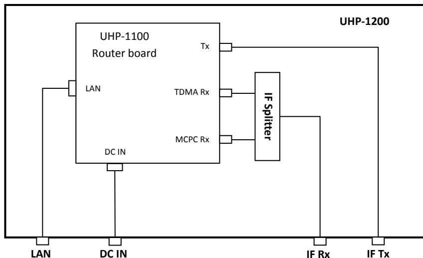
Figure 4 UHP-1200 Architecture
