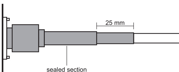
Figure 2: Sealed connector
